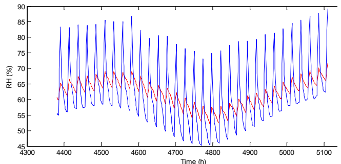
Figure 8 Interior RH(%) for Bilbao, n = 0.3 \text{ h}^{-1} , G_v = 70 \text{ g/h} , July. No MBV material (blue) and MBV = 1.3 material (red)
