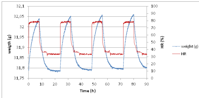
Figure 1 Moisture content evolution during MBV dynamic test
